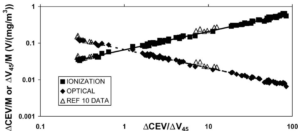
Figure 4. The sensitivities of the ionization chamber and optical scattering sensor, volts per unit gravimetric mass concentration V/(mg/m^3) , as a function of the ratio, \Delta CEV/\Delta V_{45} .
