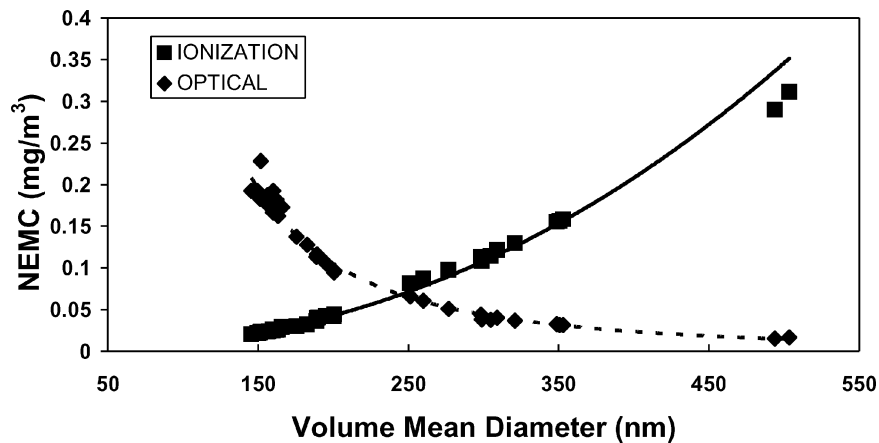
Figure 7. Noise equivalent mass concentrations (NEMC) for both the ionization chamber and the optical-scattering chamber plotted versus the volume mean diameters.
