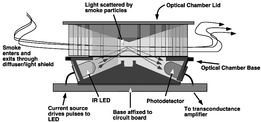
Figure 2. Schematic of the optical scattering chamber used in the dual sensors.
