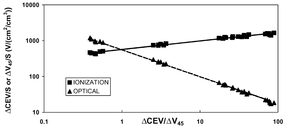
Figure 5. Correlation of ionization and optical responses per unit surface concentration with the ratio of ionization to optical response.
